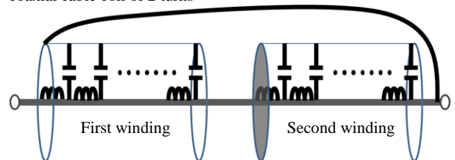
Fig.13 An Equivalent circuit of coaxial cable coil of 2 turns
