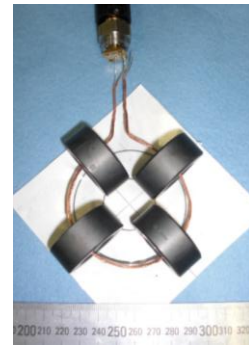
Fig.10 Photograph of device with ferrite
