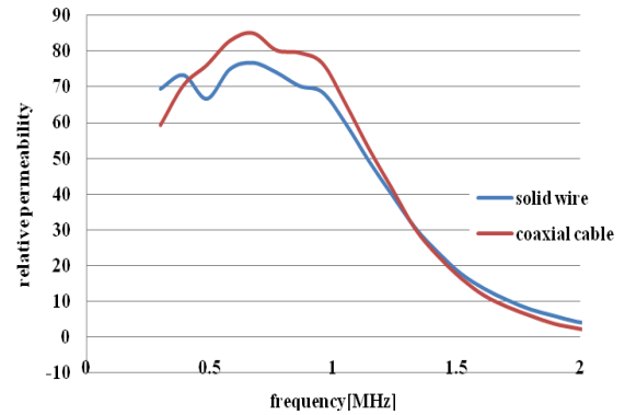
Fig.16 Relative permeability of device with ferrite core as a function of frequency
