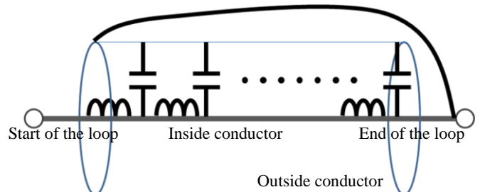
Fig.7 An equivalent circuit of coaxial cable coil of 1 turn
