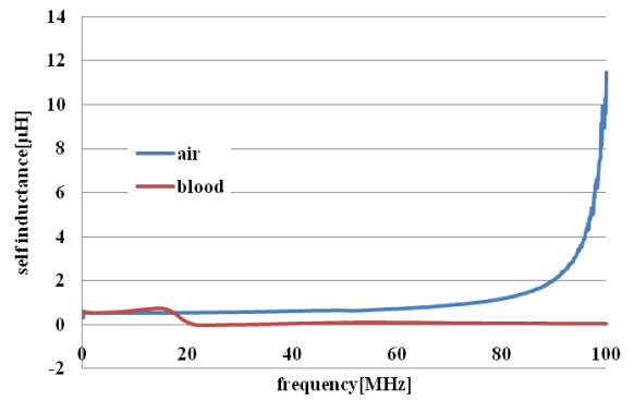
Fig.5 Self inductance with and without pig blood as a function of frequency
