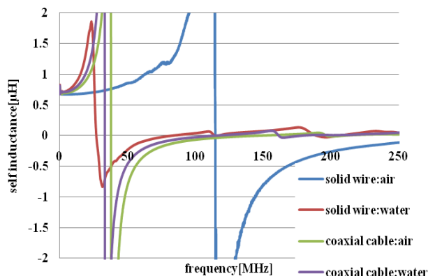
Fig.15 Self inductance with and without water as a function of frequency
