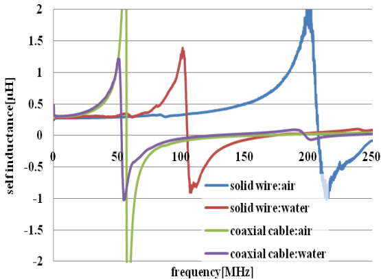
Fig.9 Self inductance with and without water as a function of frequency
