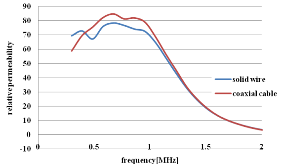
Fig.11 Relative permeability of device with ferrite as a function of frequency
